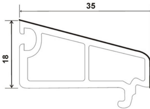
SP-60-CB , BEAD CASEMENT SINGLE GLASS (18*35)
