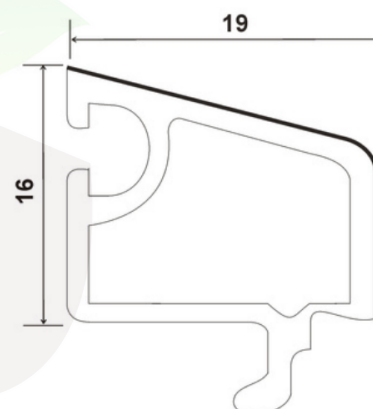
SP-88-B , SLIDING SINGLE GLASS BEAD (16*19)
