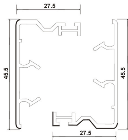
SP-88-IL, INTERLOCK WINDOW (27.5*42.5)
