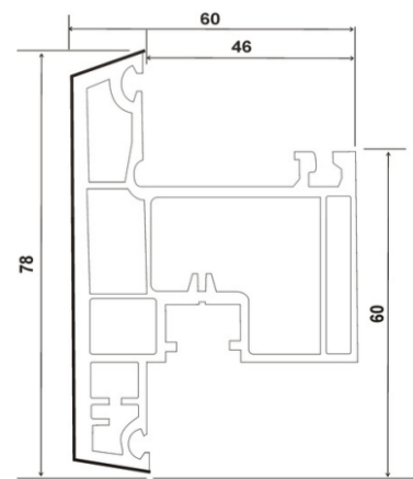
SP-60-WOS , SASH WINDOW OUTWARD (60*78)
