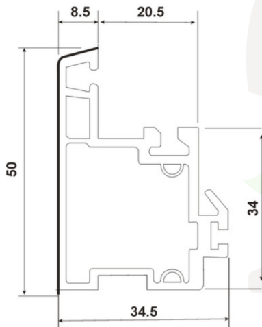
SP-61-ZT, MULLION MONORAIL (34.5*50)
