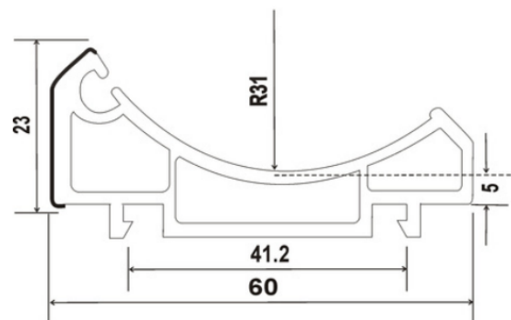
SP-WXZJ , ADAPTOR BAY POST 62MM
