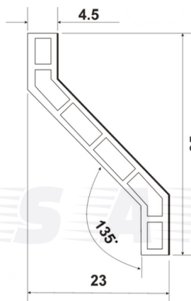
SP-BYP , LUWAR BLADE
