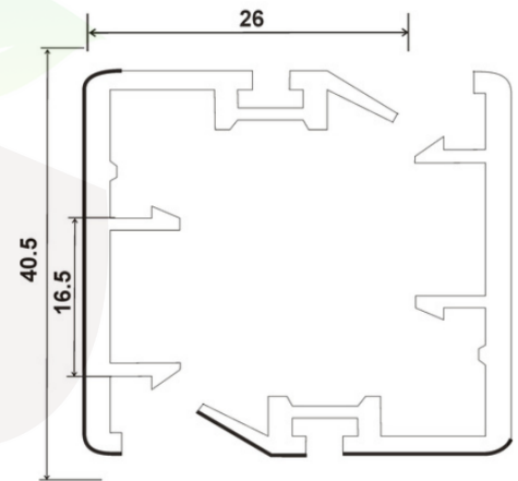
SP-80-MRIL, INTERLOCK MONORAIL (26*40.5)
