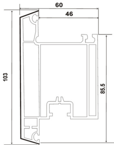
SP-60-CDS , SASH CASEMENT OUTWARD DOOR (60*103)
