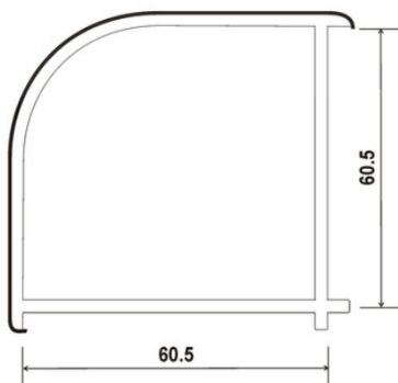
SP-60-CP , ADAPTOR SQUARE POST
