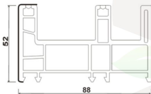
SP-88-DT , SLIDING 2.5 TRACK FRAME (88*52)
