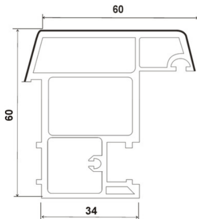
SP-60-MCM , MULLION CASEMENT MOVABLE (60*60)
