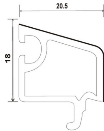
SP-60-CBS , BEAD DOUBLE GLASS CASEMENT (18*20.5)
