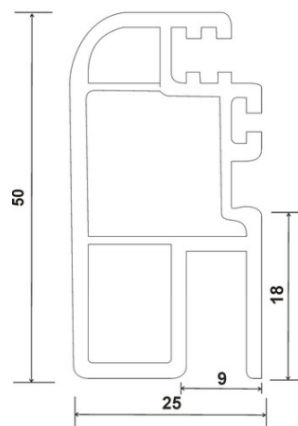
SP-80-88-MSS, SASH FLY MESH PROFILE
