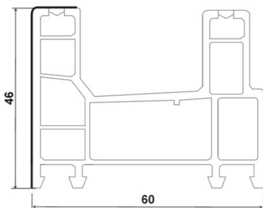
SP-60-EF , SLIDING FRAME 2 TRACK (60*46)
