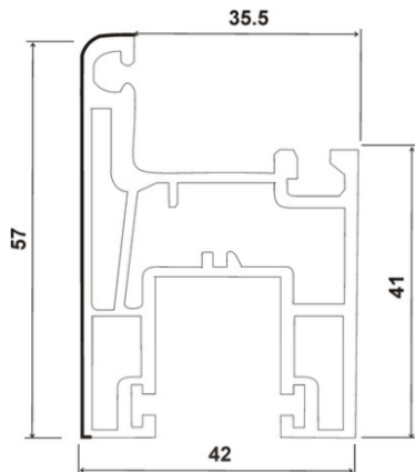
SP-88-S, SASH SLIDING WINDOW (42*57)
