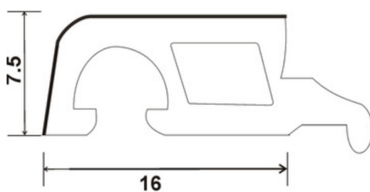
SP88-SB, DOUBLE GLASS BEAD
