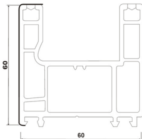
SP-60B , SLIDING 2 TRACK FRAME (60*60)
