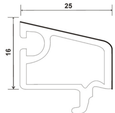
SP88-B, SLIDING SINGLE GLASS BEAD (16*25)
