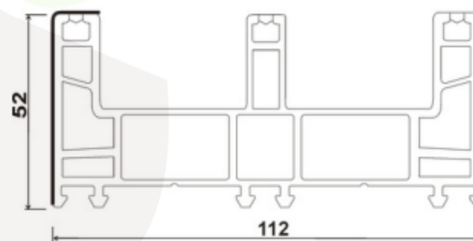
SP-112-B , SLIDING 3 TRACK FRAME (112*52)
