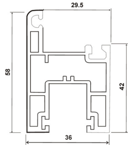
SP-80-MRS, SASH MONORAIL SLIDING (36*58)
