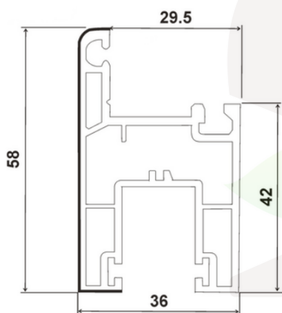
SP-60-SS , SASH SLIDING WINDOW (36*58)
