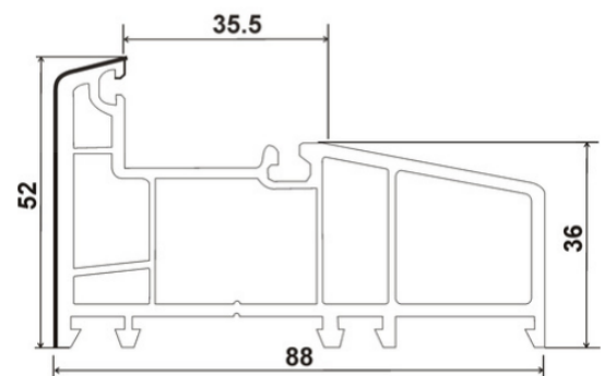
SP-88-DTF, SLIDING 2.5 TRACK FIXED FRAME
