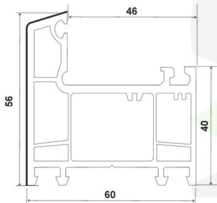
SP-60-CF , FRAME CASEMENT WINDOW (60*58)
