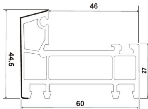
SP-60-CSF , FRAME CASEMENT NARROW (60*44.5)
