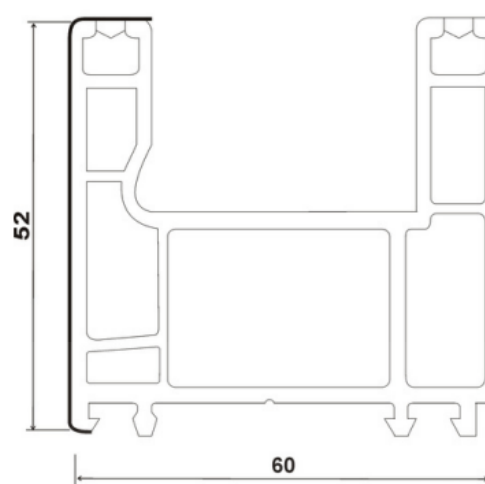
SP-60-F , SLIDING 2 TRACK FRAME (60*52)
