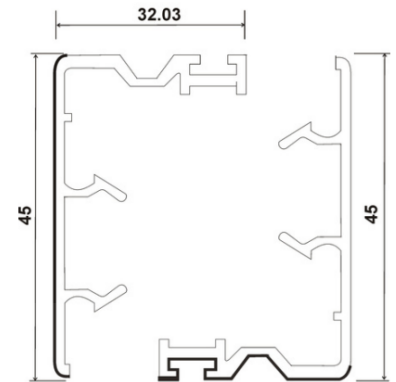
SP-95-IL, INTERLOCK WINDOW SASH
