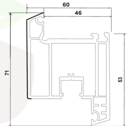
SP-60-WIS , SASH WINDOW INWARD (60*71)
