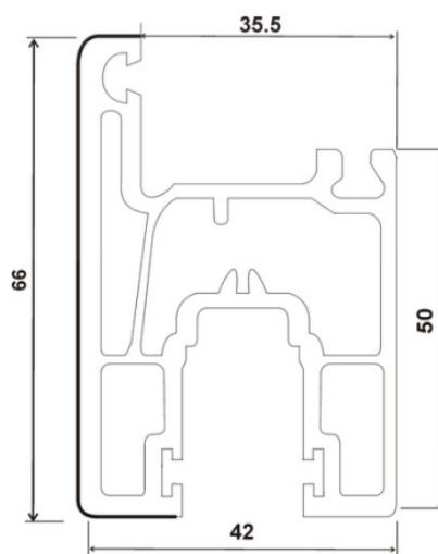
SP-95-B , SASH SLIDING WINDOW (42*66)
