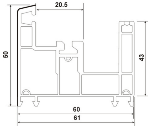
SP-61-K, SLIDING MONORAIL FRAME (61*50)
